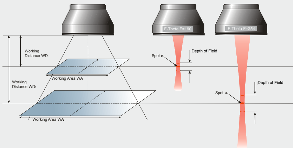
STANDARD 1064 NM F-THETA LENS
